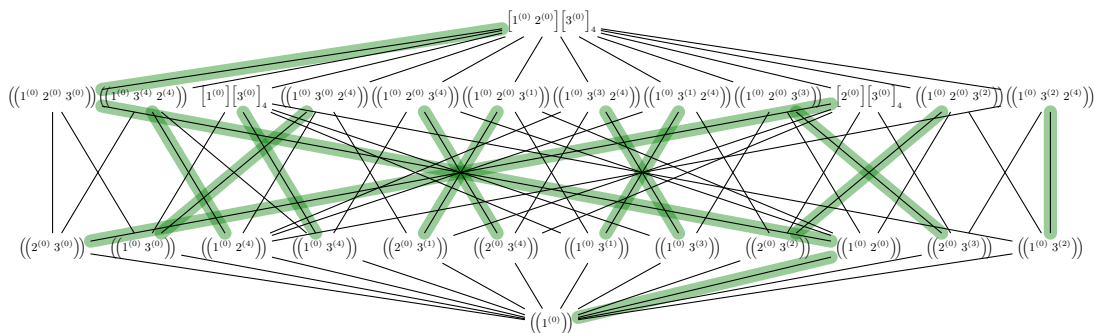
Fig. 3: The lattice \mathcal{NC}_{G(5,5,3)}\left(\left[1^{(0)} 2^{(0)}\right]\left[3^{(0)}\right]_4\right) . The symmetric chain decomposition coming from (5) is highlighted.
