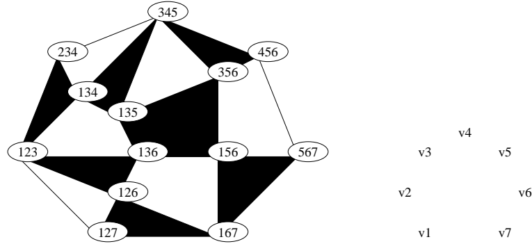
Fig. 1: Example of a plabic tiling
