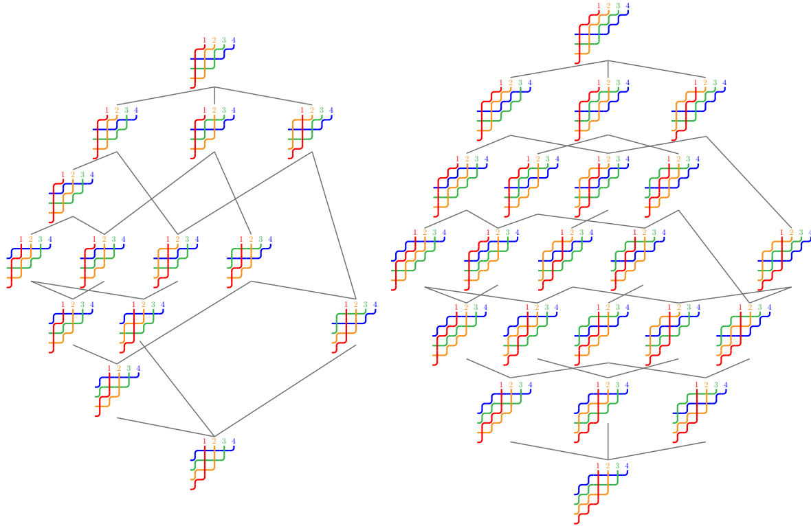
Fig. 4: The increasing flip order on (k, 4) -twists for k = 1 (left) and k = 2 (right).
