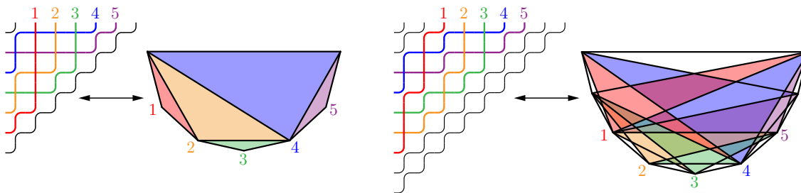
Fig. 2: Duality between (k, n) -twists and k -triangulations of the (n + 2k) -gon. Illustrated for n = 5 and k = 1, 2 .
