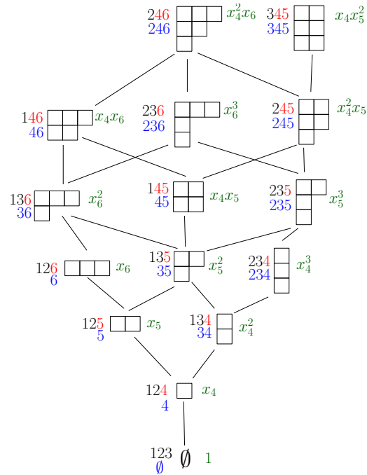
Fig. 1: An order ideal of the Young lattice
