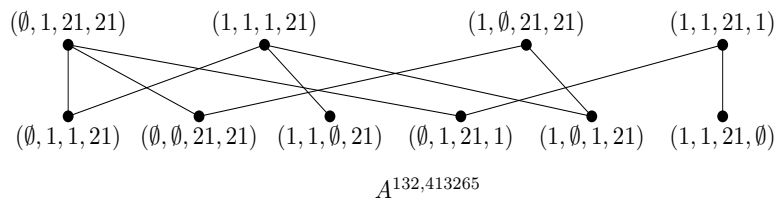
Fig. 1: The posets of the embeddings of 132 in 413265 and the union A^{132,413265} of their interiors.
