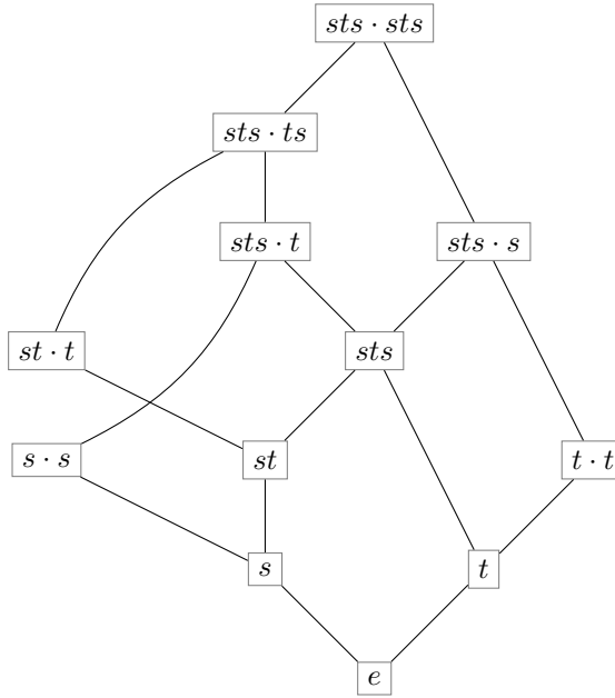
Fig. 4: \text{Camb}_{\text{Sort}}^{(2)}(A_2, st) .
