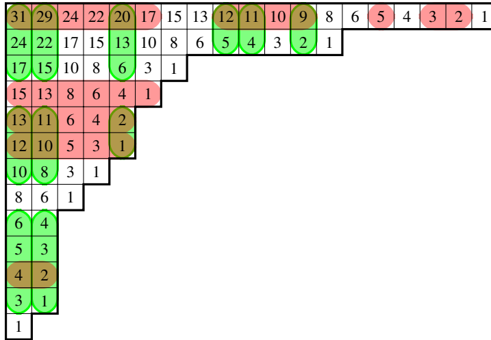
Fig. 1: A simultaneous core \kappa \in \mathfrak{C}_{7,16} with the multisets H_{7,16}(\kappa) in red and H_{16,7}(\kappa) in green.
