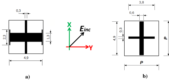
Fig. 3: Designed cells (all the dimensions are in mm.)
