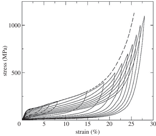
Figure 1. Experimental behaviour of EDM3 under simple (dashed line) and cyclic (solid line) oedometric compression tests.
