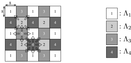
Figure 2: The four lattices \Lambda_1, \Lambda_2, \Lambda_3 and \Lambda_4 , used for embedding.
