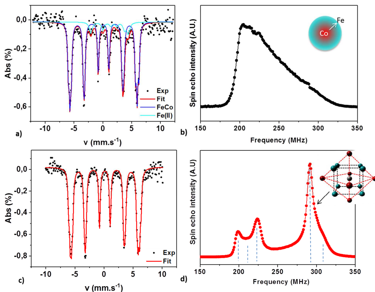
Figure 2: a-c) 5\text{K } ^{57}\text{Fe} Mossbauer spectrum and b-d) ^{59}\text{Co} Ferromagnetic Nuclear Resonance spectrum of the a-b) FeCo-PA and c-d) FeCo-HDAHCl nanoparticles. As inset, schematic view of the gradient profile determined for PA NPs and B2 order for the HDAHCl NPs (Fe : blue, Co : red) . Dashed lines are guides for the eyes for the different contributions on FeCo-HDAHCl FNR spectrum.
