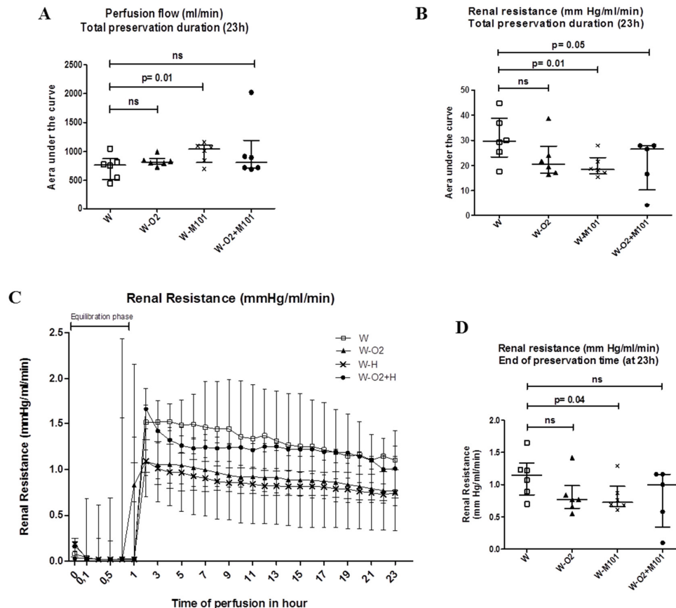
Figure 1. Ex vivo perfusion parameters. Area under the curve (AUC) representations of perfusion flow (A) and renal resistance during 23 h of cold preservation in machine perfusion (MP) Waves ® (B). Time evolution of renal resistance during 23 h of cold preservation in MP Waves ® (C) and at end of preservation time (D). Of note, the initial, "no resistance" phase (first hour, panel C) corresponds to the set-up and temperature equilibration phase of the machine (no kidney graft mounted). Results are expressed as median and interquartile range (IQR); statistical analysis was performed with Kruskal-Wallis Multiple comparison Dunn's test. n = 5-6 /group.
