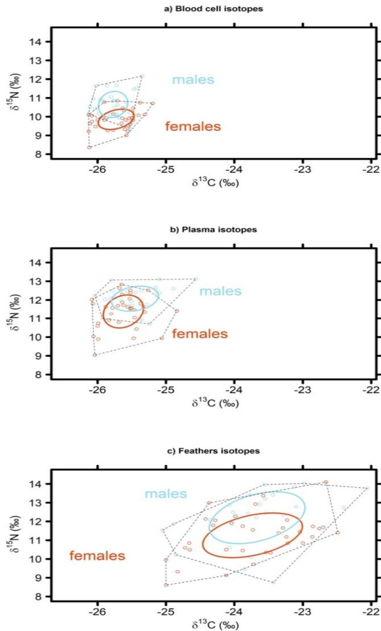
Figure 4. Isotopic niche area based on stable isotope values ( \delta^{15}\text{N} and \delta^{13}\text{C} ) in blood cells (top), plasma (middle) and body feathers (bottom) of male (blue) and female (red) snow petrels breeding at Ile des Pétrels, Pointe Géologie, Antarctica during the incubation period. The areas of the standard ellipses are represented by the solid lines, and the layman metric of convex hull area by black dotted lines.
