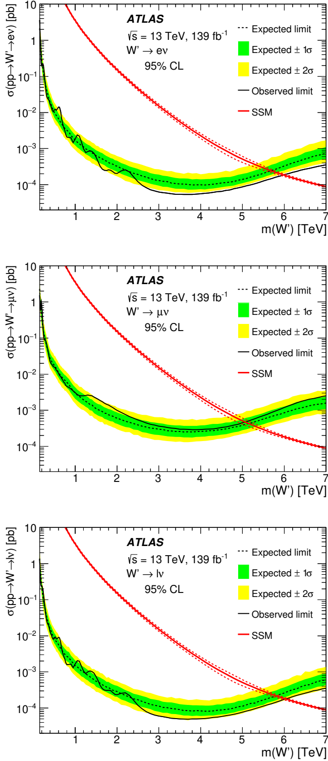
Figure 2: Observed and expected upper limits at the 95% CL on the pp \rightarrow W' \rightarrow \ell\nu cross section in the electron (top), muon (middle), and combined (bottom) channels as a function of W' mass in the Sequential Standard Model. The dashed lines surrounding the SSM cross-section curve (solid line) correspond to the combination of PDF, renormalization, and factorization scale uncertainties (for illustration only).
