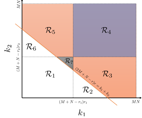
Fig. 3: Example of recovery regions imposed by the fundamental limit for the recovery of the matrices \mathbf{M}_1 , \mathbf{M}_2 and \mathbf{M} .
