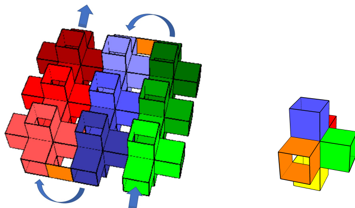
(a) A Menger inner plane and, in orange, the exterior faces used to link two lines.
