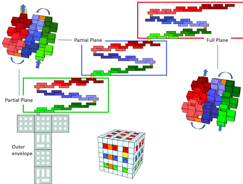
Fig. 6: The unfolding of the level 1 (3, 3, 3) -Menger polycube.
