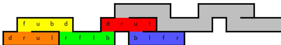
(c) The unfolding of a 5-branch cross inner line. The red branch is used to link this 5-branch cross to the next one (in grey).
