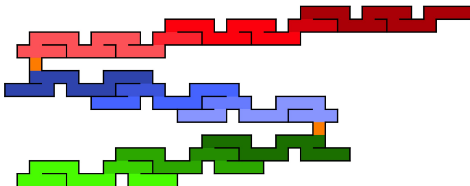
(d) The unfolding of an inner (3,3,1)-Menger plane. Faces of a same colour are from the same cross. Orange faces are outer faces.
