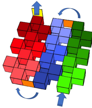
(a) A Partial Inner Plane Missing Every Top Branches.
