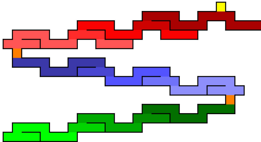
(b) The unfolding of a partial plane of a (3, 3, N) -Menger inner volume. The yellow face will be used to link this partial inner plane to one above it.
