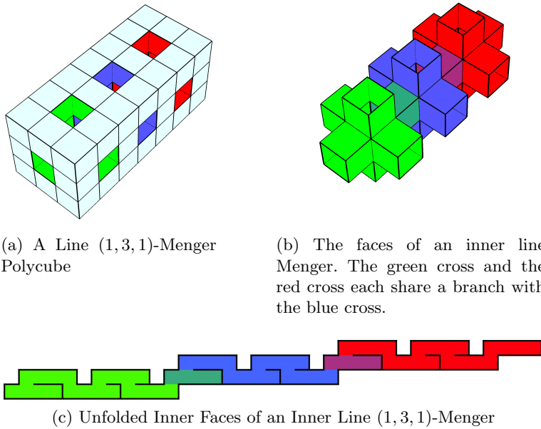
Fig. 2: The line (1,3,1)-Menger polycube. The inner faces of this polycube and its deterministic edge-unfolding.
