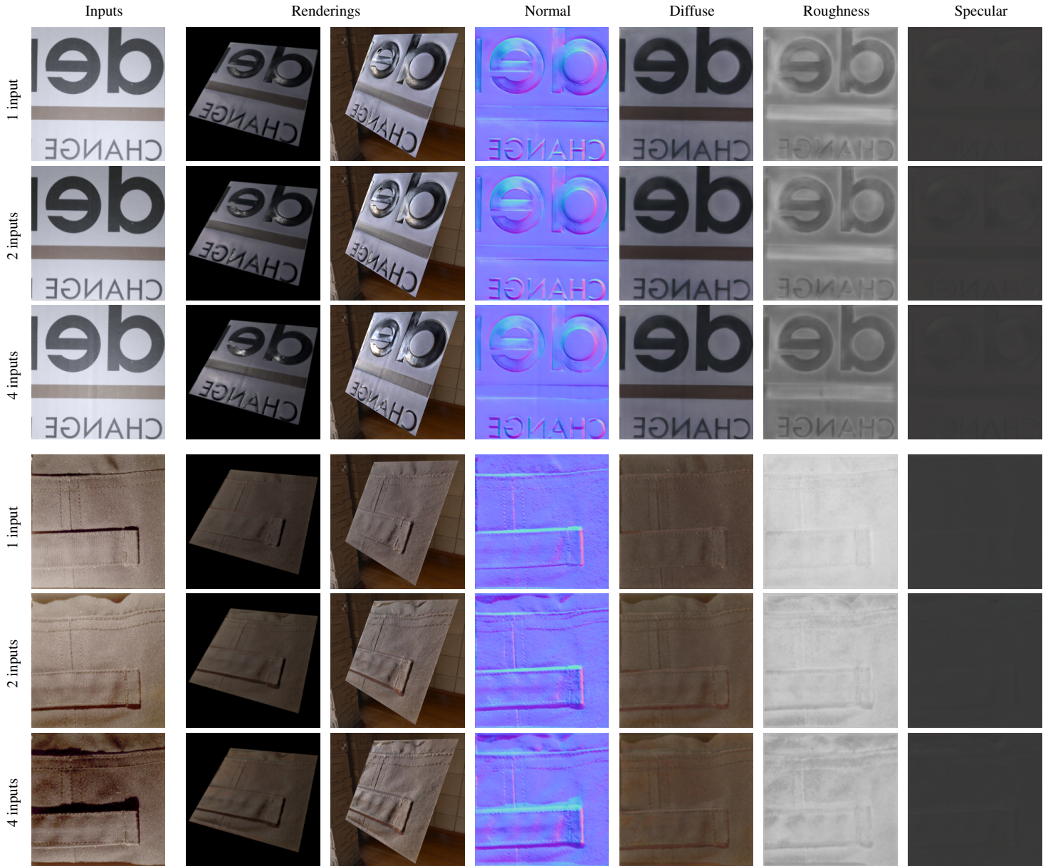
Figure 13: Limitations. We inherit some of the limitations of the method by Deschaintre et al. [DAD* 18], such as the tendency to produce correlated maps and to interpret dark pixels as shiny (top). Our SVBRDF representation, training data and loss do not model cast shadows. As a result, shadows in the input pollute some of the maps (bottom).
