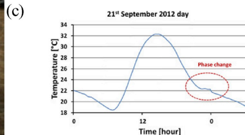
Fig. 17. (a) Test cell, (b) Schematic view of the roof, and (c) Temperature evolution of the roof [125]. Copyright (2019), with permission from Elsevier.
