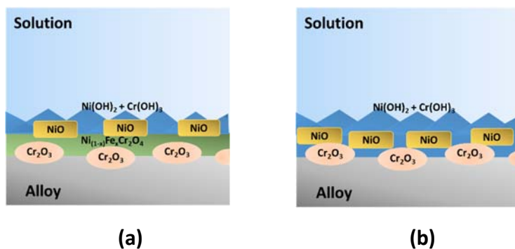
Figure 14: Model of the passive film formed on the AR (a) and MP (b) Alloy 690 in a borate buffer solution (pH 9.0) at ambient temperature
