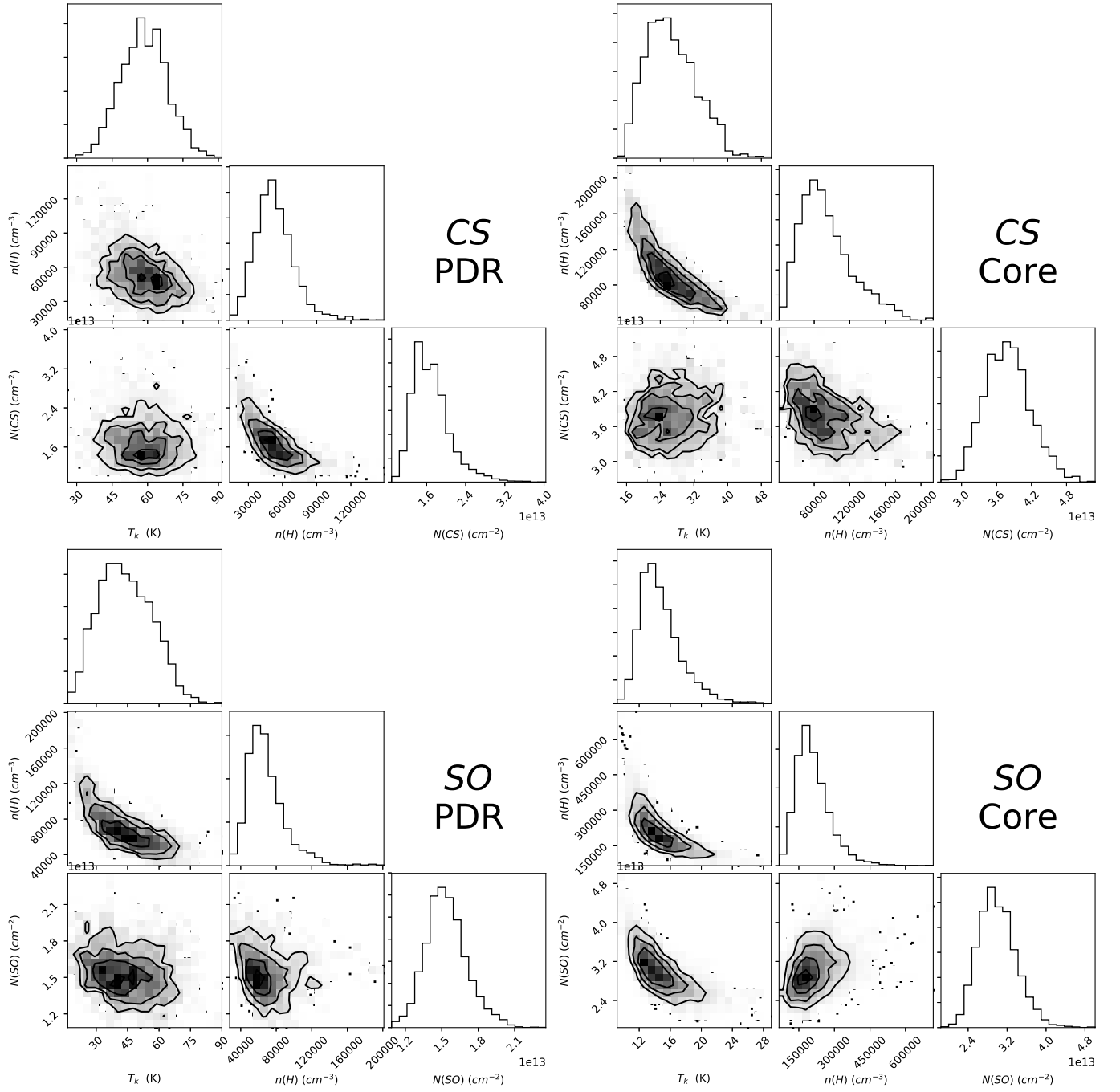
Fig. B.1. Histograms of the MCMC RADEX parameter distribution for the different molecules and regions studied.
