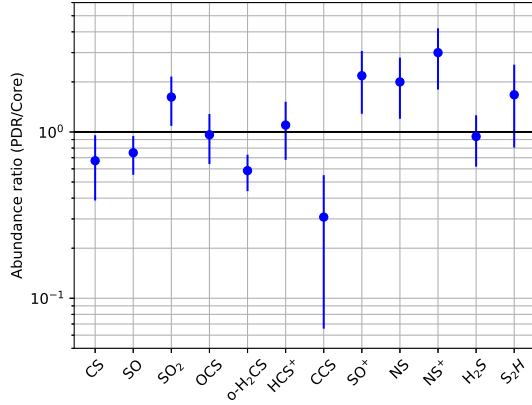
Fig. 3. Ratio between the abundance in the PDR/core position for each species.
