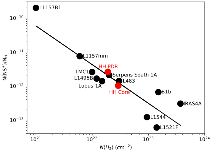
Fig. 5. Abundances of NS + as a function of N(\text{H}_2) . Black points corresponds to the detections reported by Cernicharo et al. (2018). Red points corresponds to the core and PDR positions in the Horsehead. The black solid line depicts a linear fit to the data.
