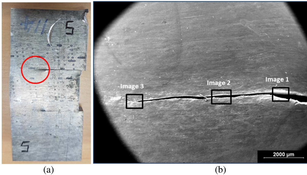
Fig.24 : (a) Post impacted AA 2024 double notch plate at 114\text{m.s}^{-1} (b) Macroscopic view of crack after surface polishing
