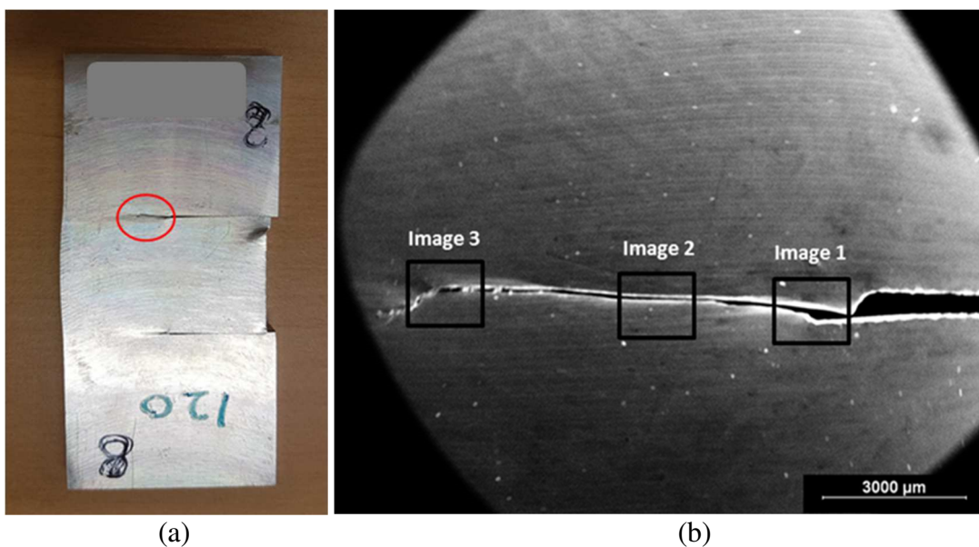
Fig.26 : (a) Post impacted AA 7175 double notch plate at 120\text{ m.s}^{-1} (b) Macroscopic view of crack after surface polishing
