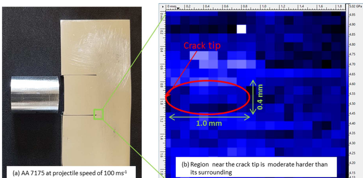
Fig.39 : Nanohardness of crack tip for AA 7175 at impacted speed of 100 m.s -1 . Light blue for higher hardness value and dark blue for lower hardness value.
