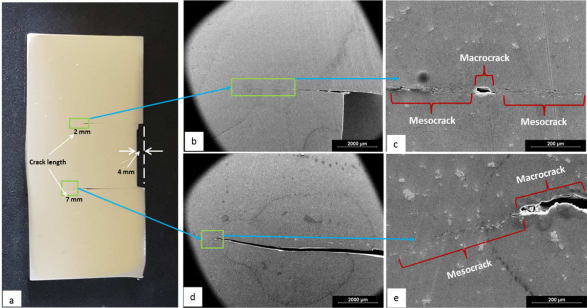
Fig.20 : Post-mortem AA 2024 specimen after impact at 111 m.s -1
