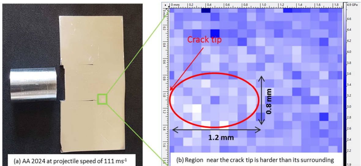
Fig.37 : Nanohardness of crack tip for AA 2024 at impacted speed of 111 \text{ m.s}^{-1} . Light blue for higher hardness value and dark blue for lower hardness value.
