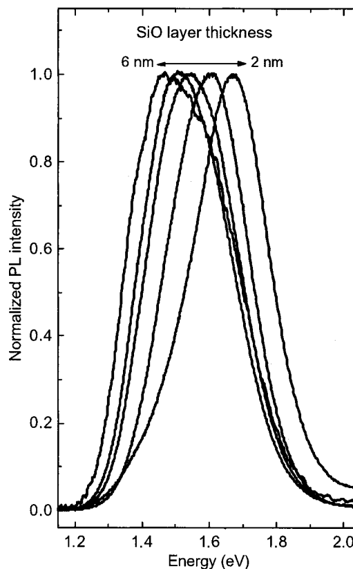
FIG. 3. Normalized photoluminescence spectra for the annealed samples with different SiO thicknesses.
