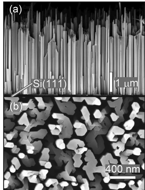
FIG. 1. (a) Side and (b) top views of an undoped sample grown on a Si substrate by using plasma assisted MBE. Length and diameter of NWs were 1\text{--}2 \mu\text{m} and about 200 nm, respectively.
