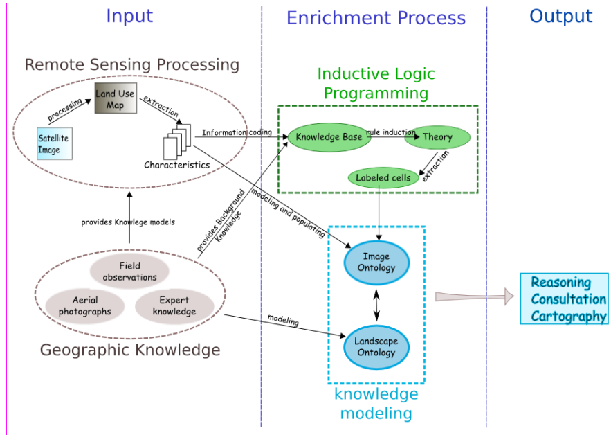
Fig. 1 Overall approach
