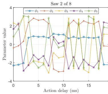
Figure 1: An example showing the instability of the estimated phase features \phi_i from measurements of the same appliance: “an electric saw” from the COOLL dataset. The x-axis represent different action delays (0 to 19 ms) i.e. different measurements of the same appliance. Between action delays the mains frequency is likely to slightly vary which affects the phase estimates.
