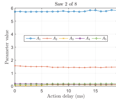
Figure 2: An example showing the stability of the estimated amplitude features A_i from measurements of the same appliance: “an electric saw” from the COOLL dataset. The x-axis represent different action delays (0 to 19 ms) i.e. different measurements of the same appliance.
