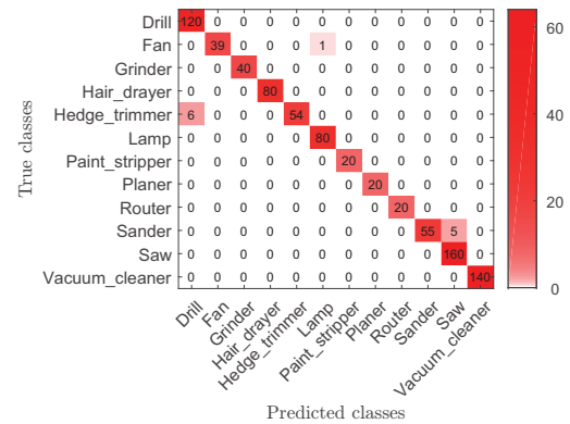
Figure 6: Confusion matrix for identification using A_i . Classification rate CR = 98.57%.
