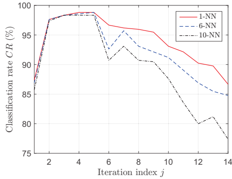
(a) CR variation corresponding to rows k = 1, 6 and 10 (representing also the number k of chosen nearest neighbors) of matrix S (Eq. (6))
