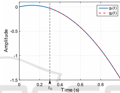
Figure 3: Functions g_1(t) and g_2(t) .
