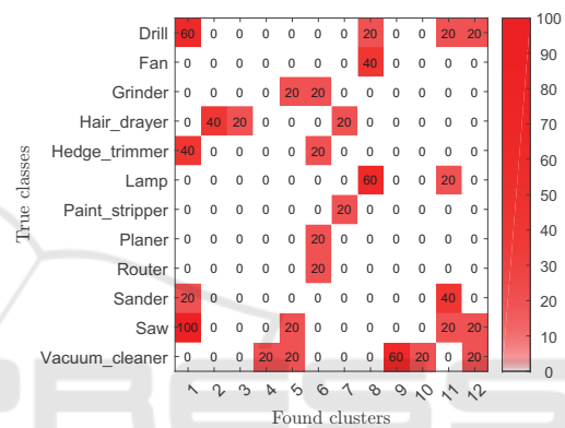
Figure 10: Confusion matrix for clustering using A_i .
