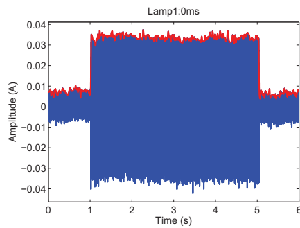
Figure 9: Turn-on transient current of a light emitting diode (LED). The interval [0, 1] s represents the pre-turn-on period whereas the interval [5, 6] s represents the post-turn-off period.
