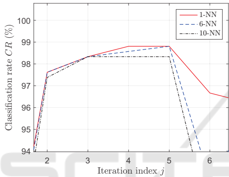
(b) Zoom of Figure 4a. The maximum values of CR for 1-NN, 6-NN and 10-NN are found, respectively, for j = 4, 5 and 3 .
