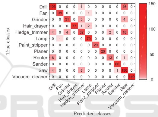
Figure 7: Confusion matrix for identification using A_0 , b_3 and A_i . Classification rate CR = 90.95%.
