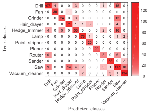
Figure 5: Confusion matrix for identification using A_0 and b_3 . Classification rate CR = 82.98%.
