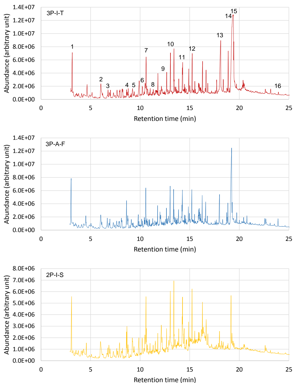
Figure 5: Py-GC/MS chromatograms of the three samples (3P-I-T, 3P-A-F, 2P-I-S).
