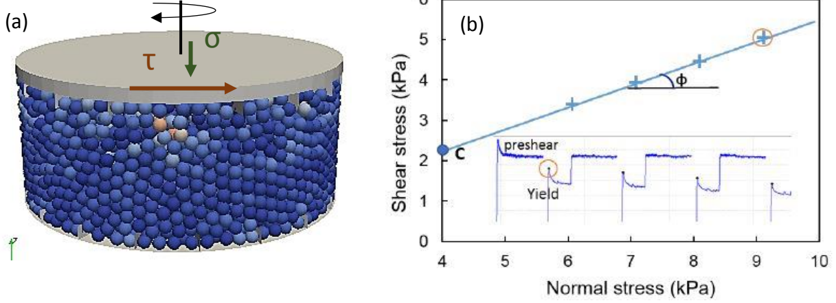
Fig. 2 (a) Snapshot of FT4 shear cell from DEM simulation. (b) Typical shear-test result showing the shear stress responses during pre-shearing and shearing and the obtained yield locus, which gives the angle of internal friction, \phi , and apparent cohesion, C .
