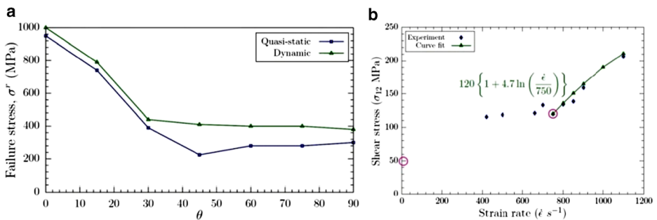
Fig. 22 a Static-dynamic comparison of failure stress versus laminate angle \theta b Shear yield stress versus strain rate, T800S/M21e laminate
