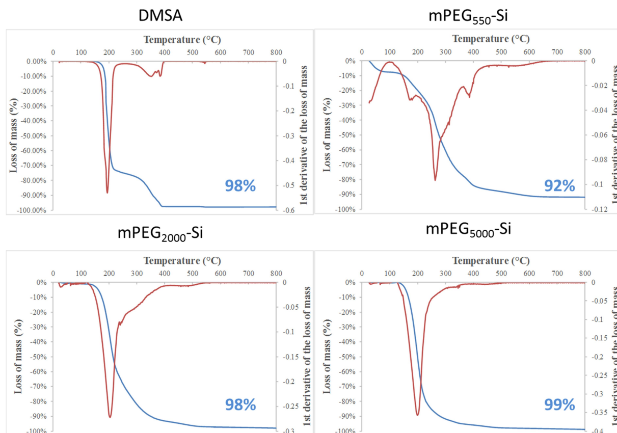
Figure S12: Thermogravimetric analyses of DMSA and mPEG x -Si (where x = 550, 2000 and or 5000 \text{ g.mol}^{-1} )
