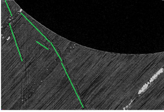
Fig. 10. Kink bands can be found in \pm 45^\circ plies when the peak strength is reached, but also before, in both UD-fabric (this picture) and woven fabric laminates.
