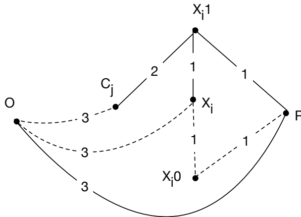
Figure 2: A schematic view of the graph G used in the reduction of Theorem 1.
