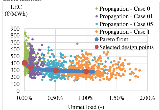
Figure 1. Pareto front and LEC and UL indicators for the four selected design configurations with uncertainties.
