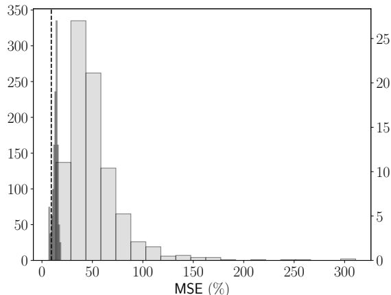
Figure 8: Histogram of the MSE sample obtained from 1000 runs of the “blindfolded” approach. The black histogram represents the 100 MSE final values (with random initialization) of Fig. 7. The black vertical dashed line represents the MSE value (12.43 %) obtained with the deterministic approach.
