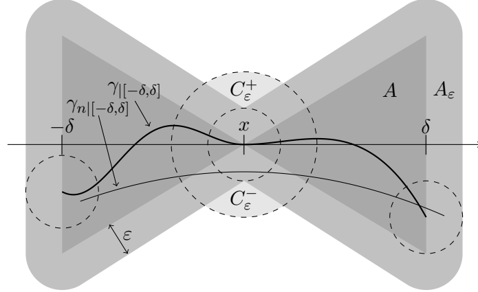
FIGURE 2. Sketch of the construction in the proof of Lemma 4.3.
