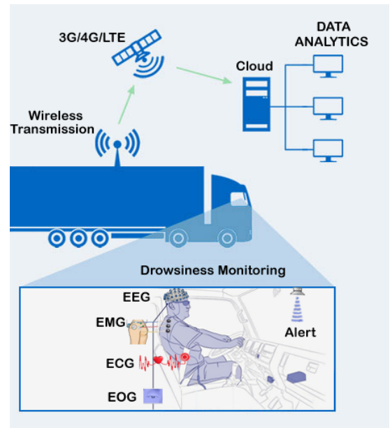
Fig. 3. Bio-Sensors Based Driver Drowsiness Detection System Architecture.
