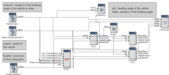
Figure 4 : Diagram of simulation with RTMaps 4.0
