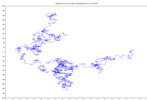
Figure 3 : Simulation of the odometric model completed
