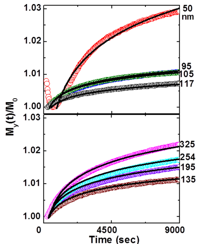
FIG. 2. Time dependence of in-plane magnetization measured at 300 K for (a) 50, 95, 105, and 117 nm and (b) 135, 195, 254, and 325 nm LSMO films. The solid lines are logarithmic fittings to the magnetization relaxation data.
