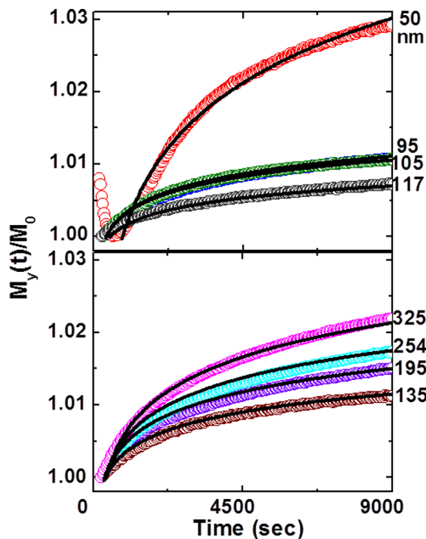
FIG. 2. Time dependence of in-plane magnetization measured at 300 K for (a) 50, 95, 105, and 117 nm and (b) 135, 195, 254, and 325 nm LSMO films. The solid lines are logarithmic fittings to the magnetization relaxation data.
