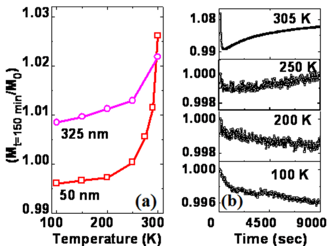
FIG. 4. (a) Temperature dependence of the total magnetization relaxation measured in 50 and 325 nm LSMO films. (b) Time dependence of magnetization of the 50 nm sample at different temperatures.
