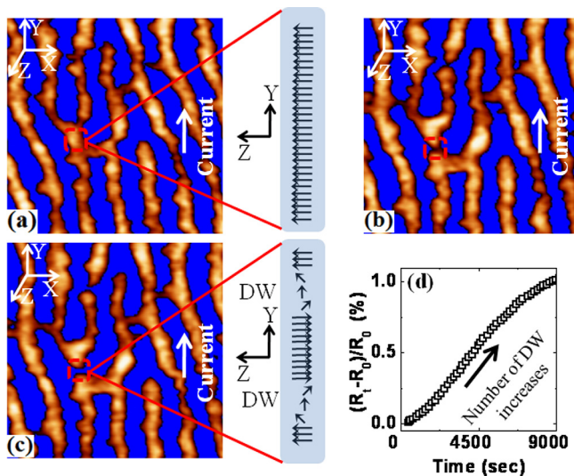
FIG. 1. MFM images (taken at the same place) of the 135 nm LSMO film at (a) 5, (b) 70, and (c) 130 min after the external magnetic field (applied along the Y direction) was switched off. The scan size is 1 \mu\text{m} \times 1 \mu\text{m} . The marked square highlights one particular case of the emergence of additional domain walls. The configurations of the DWs are shown in the schematics on the right side of the MFM images. Note that the coordinates of the schematics are different from those of the MFM images for clarity. (d) Increase of resistance with time as a result of the enhanced scattering of electrons at DWs.
