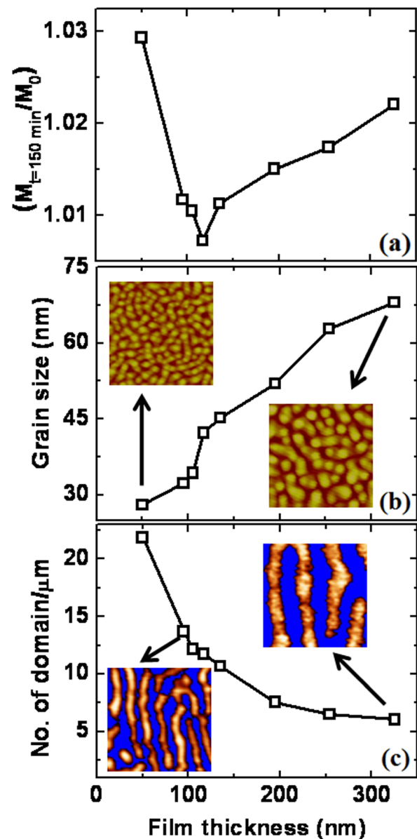
FIG. 3. (a) Thickness dependence of the total change of magnetization in LSMO films measured over 150 min. (b) and (c) show the thickness dependence of the average grain size and the number of magnetic domains per unit length along the X axis (same coordinates as in Fig. 1). The insets in (b) and (c) show the typical AFM and MFM images, respectively. The scan size is 1 \mu\text{m} \times 1 \mu\text{m} for all images.
