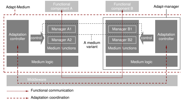
Fig. 3. Adapt-Medium architecture
