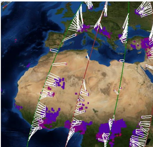
Figure 5 Example of mission plan computed by ATLAS
