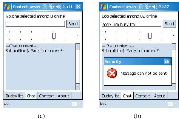
Fig. 8. Messenger interface
