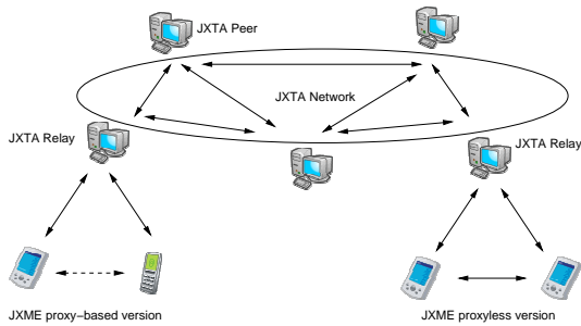
Fig. 6. JXTA and JXME network
