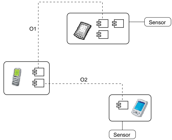
Fig. 3. p2pContext context management
