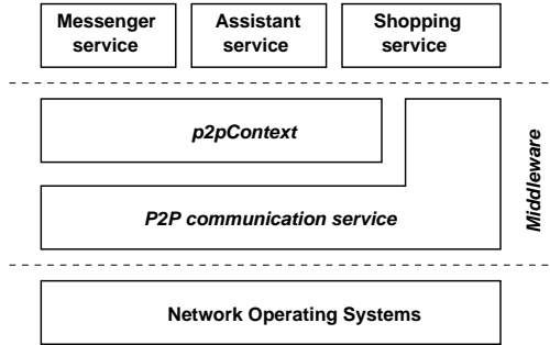
Fig. 2. Software application architecture
