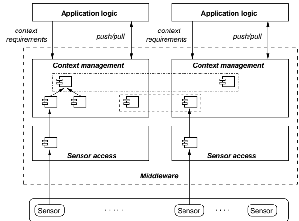
Fig. 4. Middleware architecture
