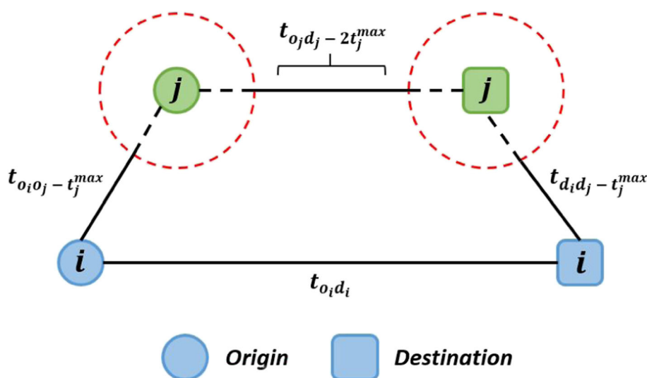
Fig. 7 Early checking - infeasibility check of a match
