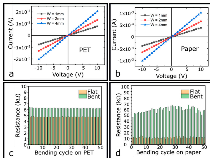
Figure 2. Electrical behaviour of the CB ink printed resistors under strain. Current versus voltage plots on (a) plastic and (b) paper substrates. Measured resistances during 50 bending cycles of the inkjet-printed CB line ( W = 4 mm) in flat and bent positions for the (c) plastic and (d) paper substrates. Bending radius was kept constant at 4 mm.
