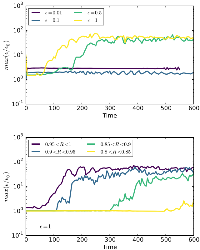
Figure 5. Top: Maximum solid-to-gas ratio \epsilon_{\max} as a function of time, relative to the initial solid-to-gas-ratio \epsilon_0 , for St = 0.1 and for different values for \epsilon . Bottom: Time evolution of \epsilon_{\max} for St = 0.1 and \epsilon = 1 at different radius bins. It shows that the instability propagates inwards because of the combined effect of particle trapping and drift.
