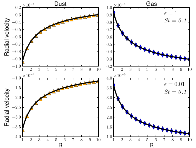
Figure A1. Radial velocity of the dust and gas components for runs aimed at testing the method to solve the momentum transfer between dust and gas through the radial drift problem. Analytical solutions given by equations (5) and (7) are plotted with the solid line, while numerical simulations are displayed with the coloured symbols.
