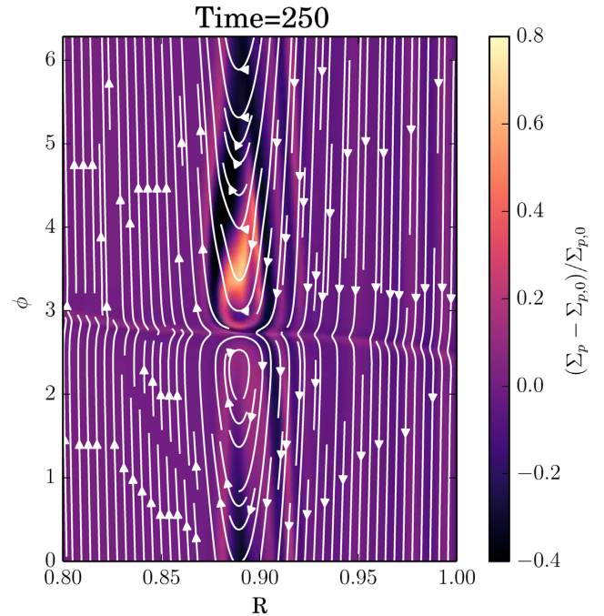
Figure 20. Streamlines and relative surface density perturbation of pebbles at Time = 250 for the simulation in which the planet is allowed to migrate.
