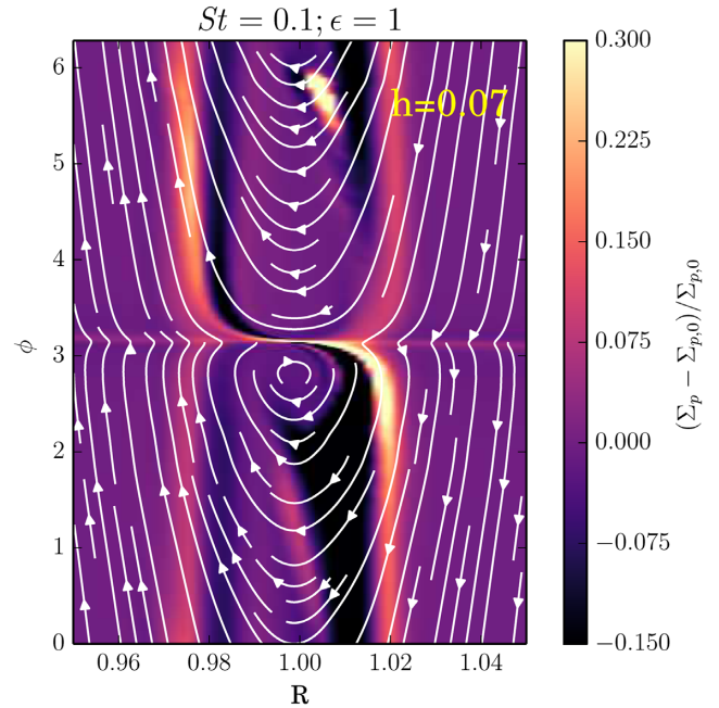
Figure 2. Streamlines and relative surface density perturbation of pebbles at Time = 50 for a simulation St = 0.1 , solid-to-gas ratio of \epsilon = 1 corresponding to a thicker disc with h \sim 0.07 . This model has therefore an effective scale height such that \tilde{H}/R = 0.05 .
