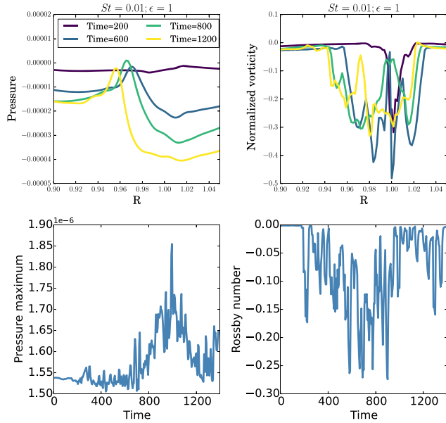
Figure 10. Top: Azimuthally averaged profile of the gas pressure at different times for \epsilon = 1 initially and Stokes number St = 0.01 ( Left ) and azimuthally averaged profile of the normalized gas vorticity at the same time ( Right ). Bottom: For the same run, time evolutions of the pressure maximum at vortex centre ( Left ) and Rossby number ( Right ).
