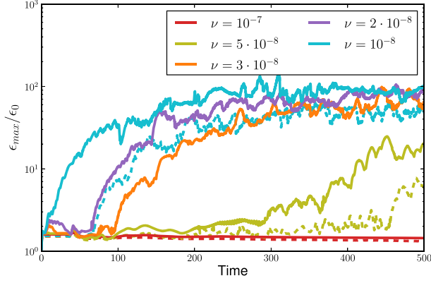
Figure B1. Maximum solid-to-gas ratio \epsilon_{\max} as a function of time, relative to the initial solid-to-gas ratio \epsilon_0 = 1 , for different levels of kinematic viscosity. The dashed lines correspond to moderate resolution runs with (N_R, N_\phi) = (848, 2000) , whereas the solid lines are for high-resolution simulations with (N_R, N_\phi) = (1696, 4000) .
