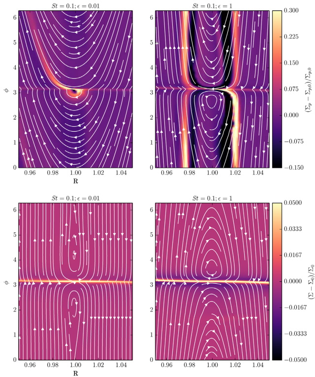
Figure 1. Top: Streamlines and relative surface density perturbation of pebbles at Time = 50 for St = 0.1 and for solid-to-gas ratios of \epsilon = 0.01 (Left) and \epsilon = 1 (Right). Bottom: Corresponding relative gas surface density perturbation and gas streamlines.
