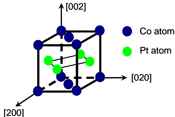
Figure 2: L1 0 ordered structure
