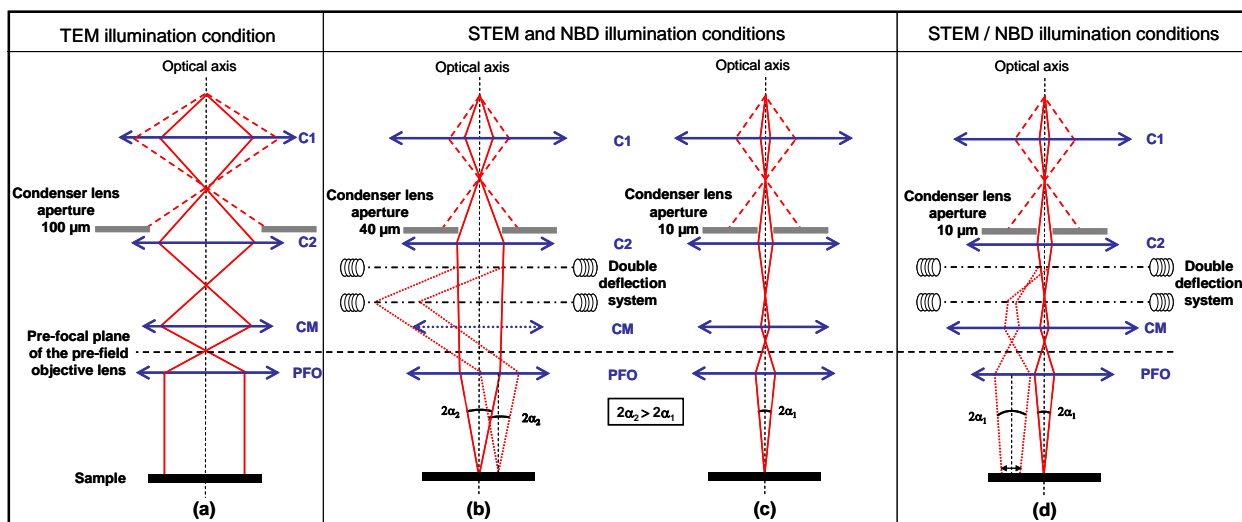
Figure 1: Ray diagrams of the illumination system (C1 and C2: Condenser lenses; CM: Condenser Mini lens; PFO: Pre-Field Objective lens). (a) Parallel beam condition in conventional TEM – (b) Conventional STEM condition – (c) Conventional NBD condition – (d) STEM / NBD condition (large dashed lines: stopped beam by the condenser aperture; dotted lines: deflected beams by the scanning system)
