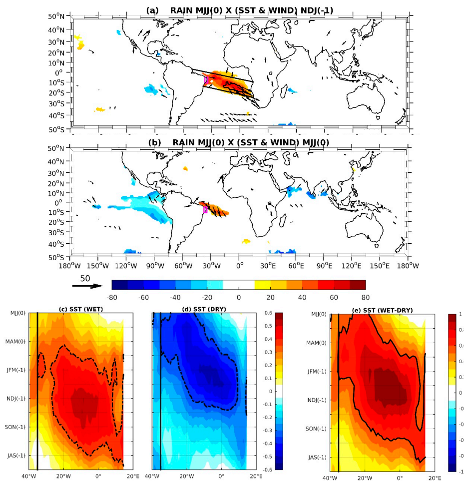
Figure 2. Distributions of the lagged linear correlation/regression ( \text{mm month}^{-1}/^{\circ}\text{C} ) of the gridded SST (from OAFlux) anomalies in (a) November–December–January(–1) (NDJ(–1)) and (b) MJJ(0) with the rainfall anomalies in Eastern NEB (magenta box) during MJJ(0) for the period 1960–2015. The vectors represent the linear regression ( \text{mm month}^{-1}/\text{m s}^{-1} ) of the surface wind vectors (u and v; from NCEP) anomalies, with the rainfall anomalies in Eastern NEB. The correlations that are significant at the 95% confidence level, according to the t -test, are plotted for both SST and wind. Contours indicate regions of correlation higher than +0.5 (solid black line) for SSTA. The diagonal band in Figure 2a indicates the pathway of the northwestward propagation of SSTA. Longitude–time diagrams of the composites of standardized SSTA for: (c) WET years, (d) DRY years and (e) difference WET–DRY years for the period 1960–2015. The SSTA are averaged along the latitude of the diagonal band in Figure 2a. Contours represent values significant at a 95% confidence level using the t -test. The vertical black lines (at 35° W) in (b–d) indicate the eastern limit of the Eastern NEB.
