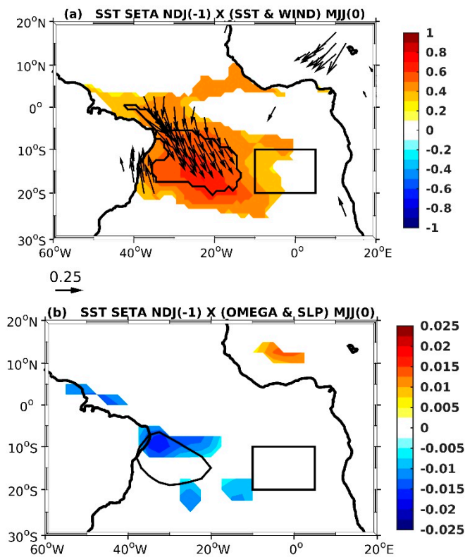
Figure 4. Distribution of the lagged linear correlation/regression of the gridded (a) SST (shaded; °C/°C) and surface wind (vectors; m s -1 /°C) anomalies (b) 500 hPa vertical velocity (shaded; Pa s -1 /°C; negative values indicate upward motion) and the sea level pressure (contours, significant correlation only) anomalies within the entire tropical Atlantic in MJJ with SSTA inside southeastern tropical Atlantic (SETA; 10° S–20° S, 10° W–5° E; oceanic black box) in NDJ for all the years (56 years) from 1960 to 2015. Only the correlations that are significant at a 95% confidence level, according to the t -test, are plotted for all variables. Contours in (a) indicate regions of correlation higher than +0.5 for SSTA.
