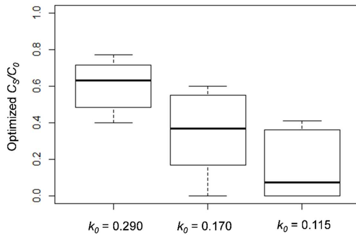
Figure 7. Variability of the initial stable C pool proportion ( C_S/C_0 ) optimized for each site ( n = 20 ) for three different values of the potential mineralization rate ( k_0 ). Boxplots show median and quartiles, while whiskers represent samples lying within 1.5 times the interquartile range. Extreme outliers are not shown.
