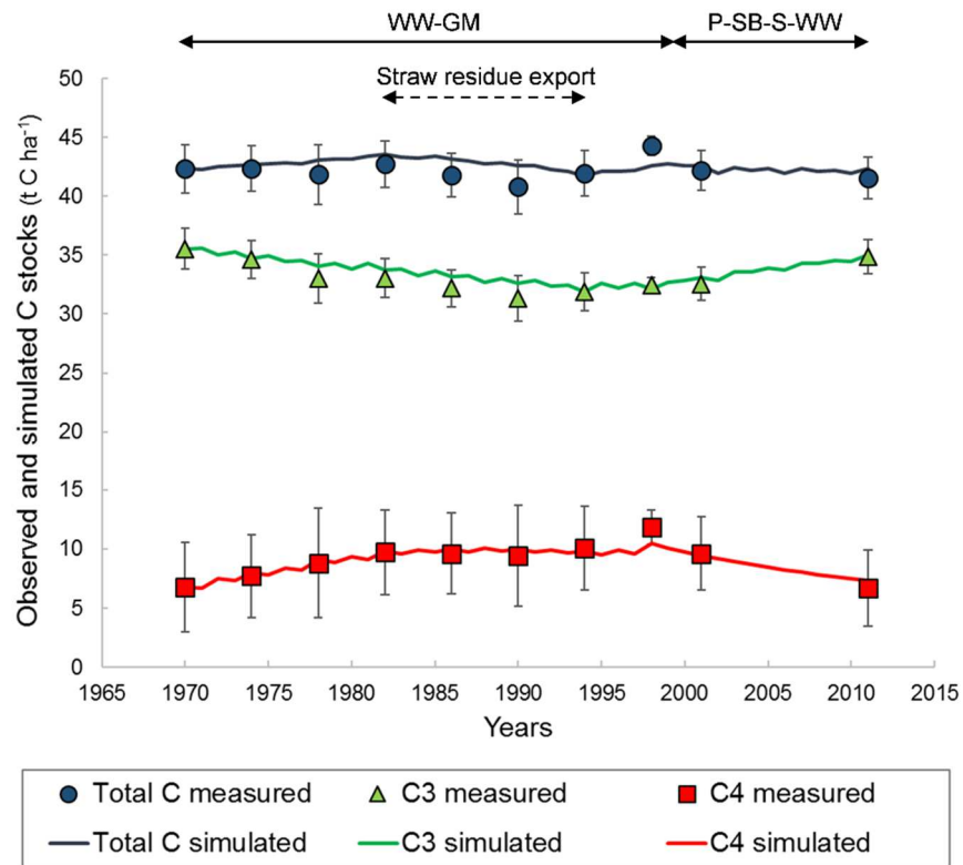
Figure 4. Example of observations (symbols) and simulations performed by AMG (solid lines) of SOC stock evolutions in the upper soil layer (29 cm depth) of one treatment of the Boigneville long-term experiment (BOIG_A_CM4_L0). Circles represent total SOC stocks, while triangles and squares represent C stocks originating from C 3 and C 4 crops, respectively. Crop abbreviations: WW = Winter Wheat, GM = Grain Maize, P = Pea, SB = Spring Barley, S = Sugarbeet. Error bars are measured SD.
