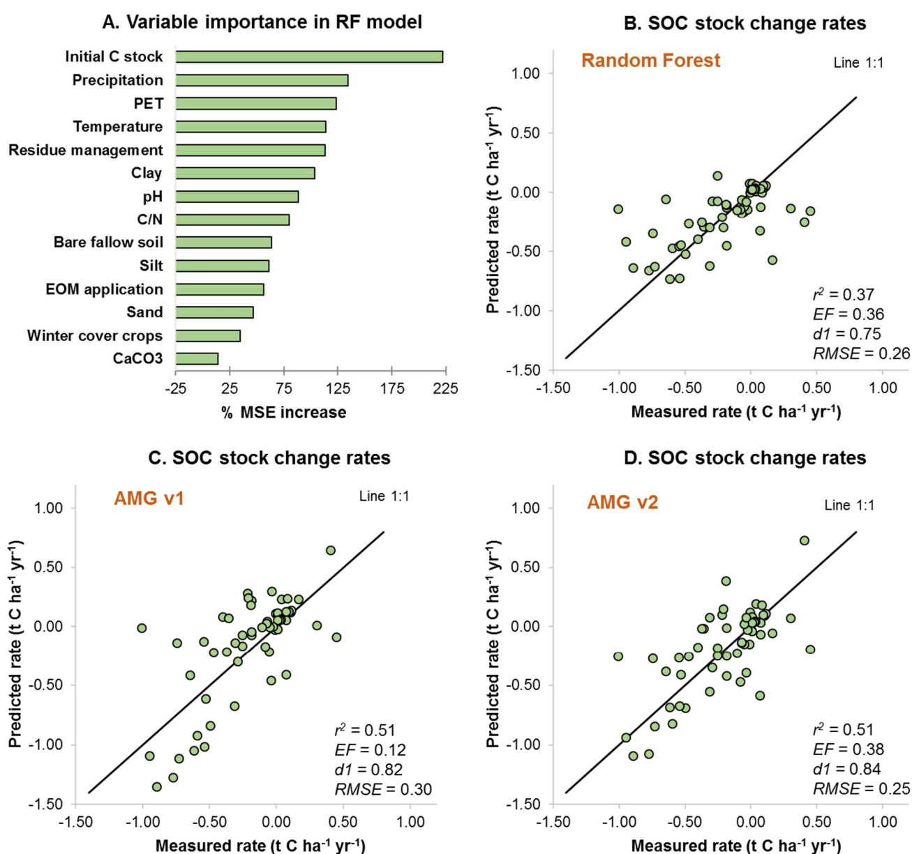
Figure 3. Variable importance in a random forest (RF) model predicting SOC stock change rates for the 60 field trials (A) and observed vs predicted variations obtained with the Random Forest (B), AMGv1 (C) and AMGv2 (D) models. SOC: soil organic carbon, EF : modeling efficiency, d1 : index of agreement, RMSE : root mean squared error of the model.
