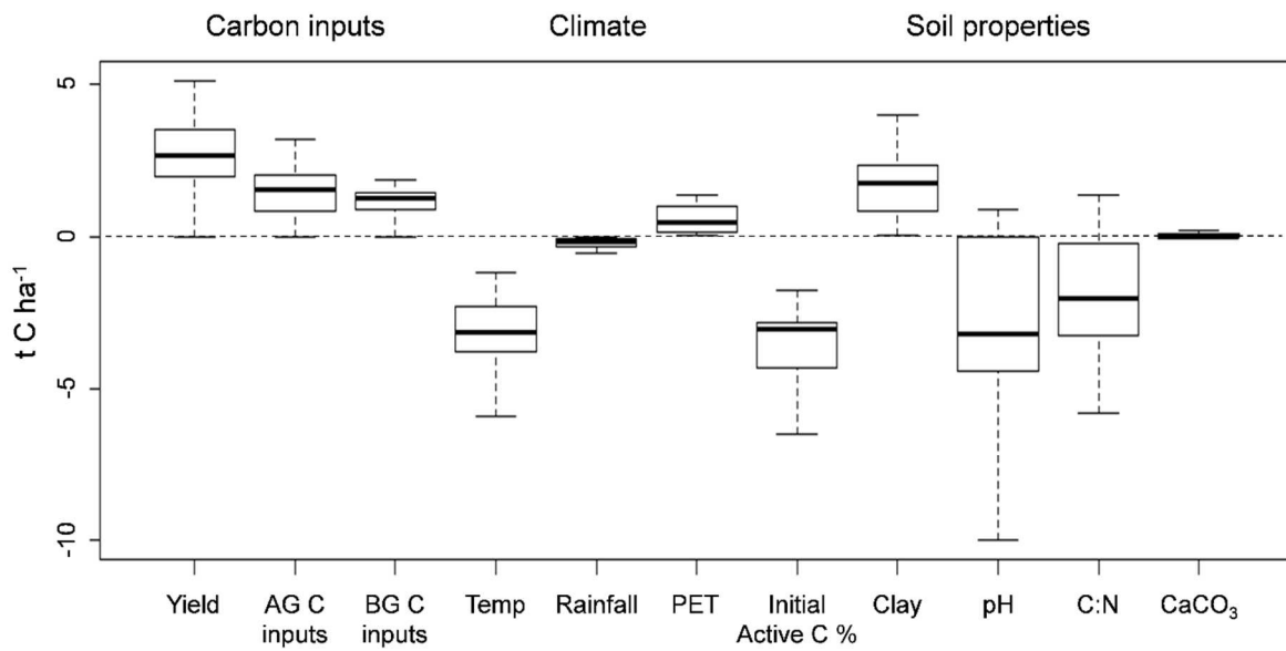
Figure 6. Boxplots showing the sensitivity of the AMGv2 model to 20% increase in different variables/parameters related to C inputs and SOM mineralization, excepting temperature and pH which were increased by 2°C and 1 pH unit, respectively. Boxplots represent the variations of the differences between the modified scenario (increase of the variable) and the reference scenario for all 60 trials over an extended period of 100 years. The dotted line represents the result for the simulation of final SOC stocks in the reference scenario with unmodified data and parameters. Boxplots show median and quartiles, while whiskers represent samples lying within 1.5 times the interquartile range. Extreme outliers are not shown.
