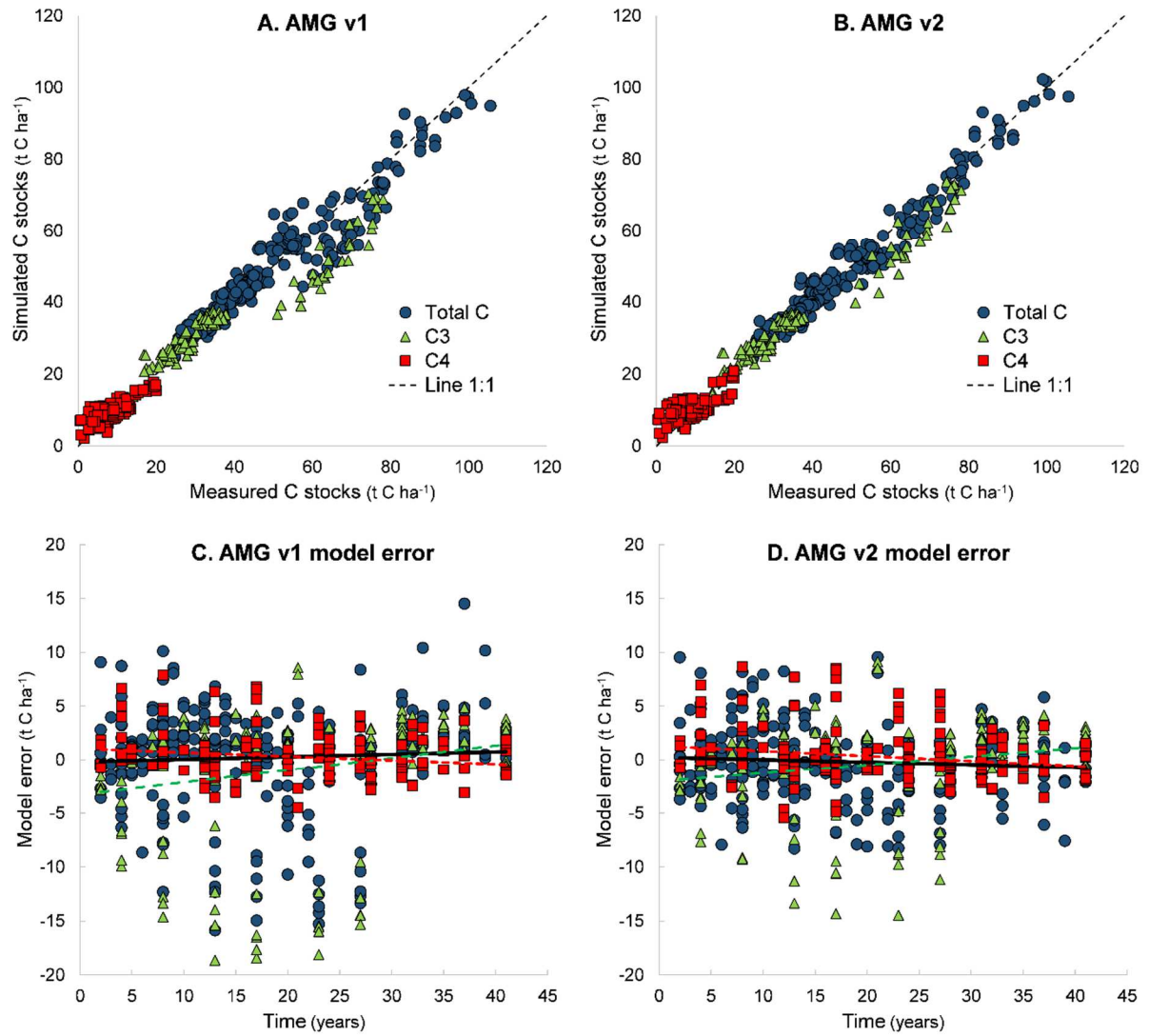
Figure 5. Measured vs predicted SOC stocks by the AMGv1 (A) and AMGv2 (B) models and error (difference between simulated and measured SOC stocks) over time of AMGv1 (C) and AMGv2 (D) for all sampling dates of the 60 field-trials. Circles represent total SOC stocks, while triangles and squares represent C stocks originating from C3 and C4 crops, respectively. The solid line represents the regression line between model error and time for total C, while the red and green dotted lines represent the regressions for C originating from C 4 and C 3 crops, respectively.
